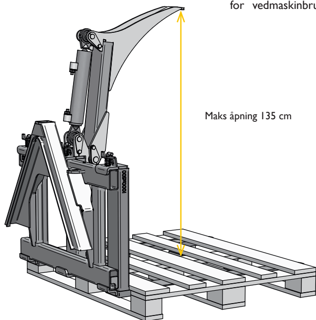
2097 / UNIVERSALKLO / 31 kg For pallegaffel / uten pallegaffel
